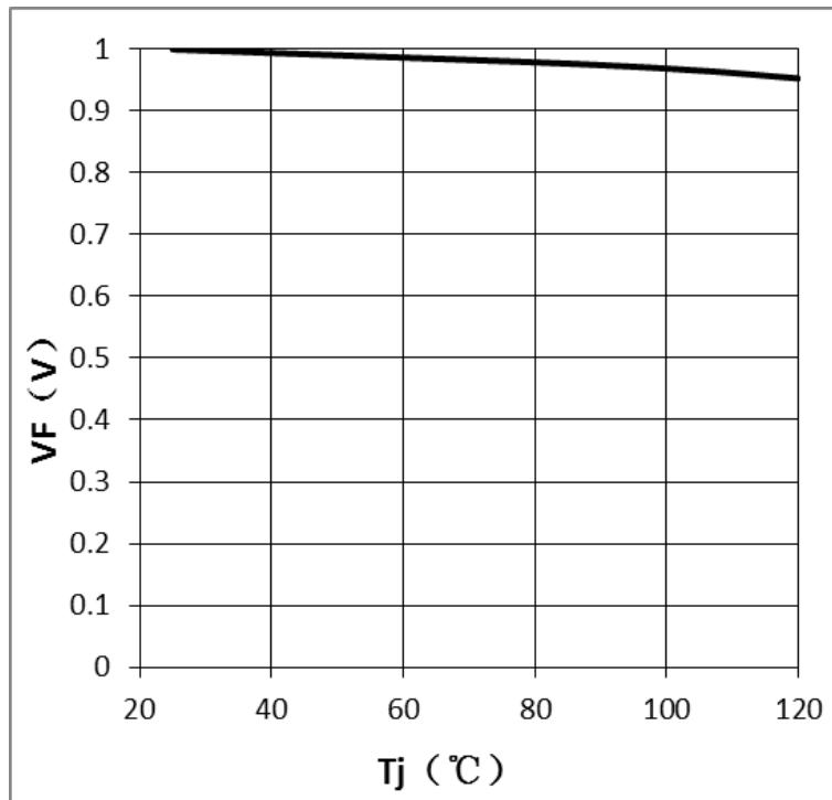
Fig 7. Junction Temperature vs. Relative Forward Voltage, I_F=65mA
