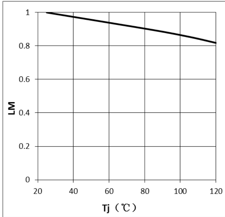
Fig 6. Junction Temperature vs. Relative Luminous FLUX , I_F=65mA
