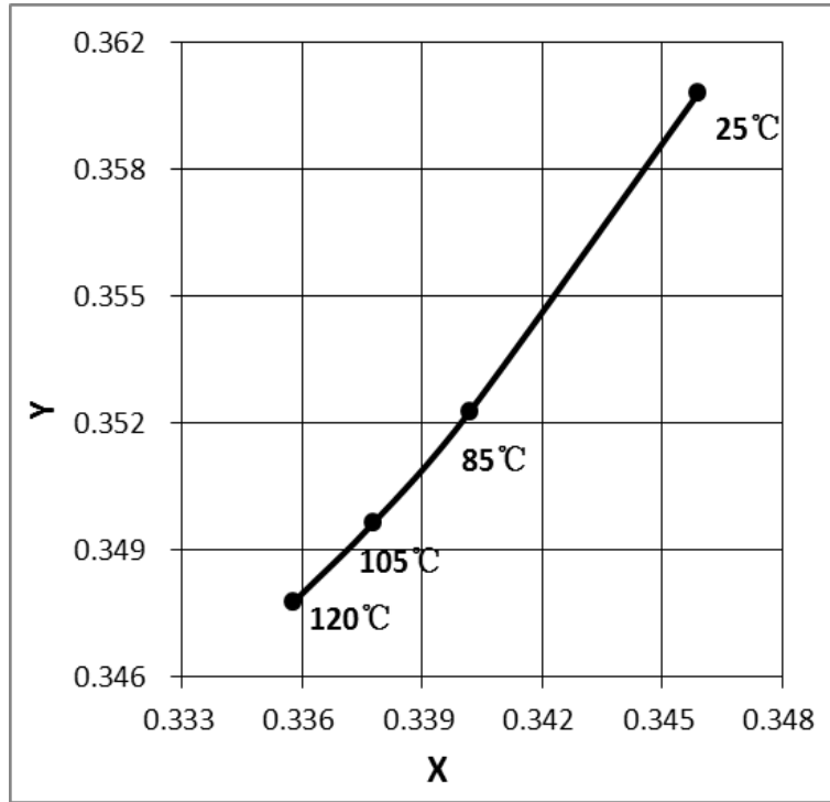
Fig 8. Chromaticity Coordinate vs. Junction Temperature, I_F=65\text{mA} (2600~4200K)
